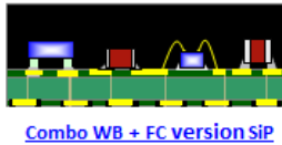
Combo WB + FC version SiP
